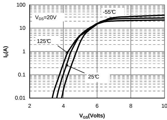
Figure 3: Transfer Characteristics
