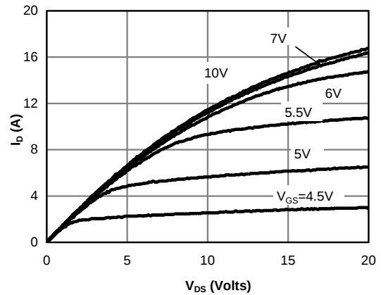
Figure 2: On-Region Characteristics@125°C
