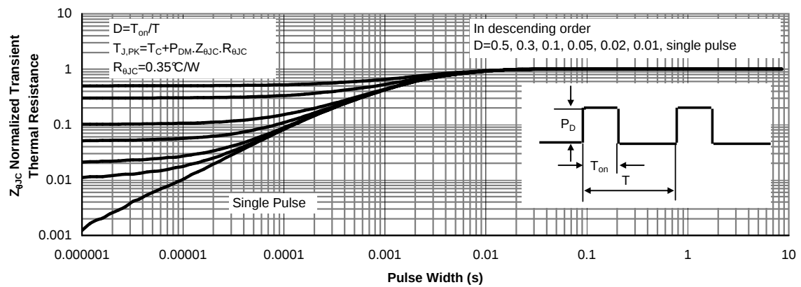
Figure 14: Normalized Maximum Transient Thermal Impedance for AOW29S50 (Note F)
