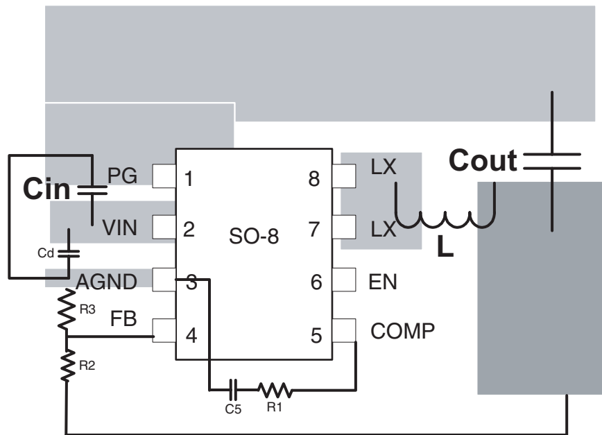
Figure 3. AOZ1075 PCB Layout
