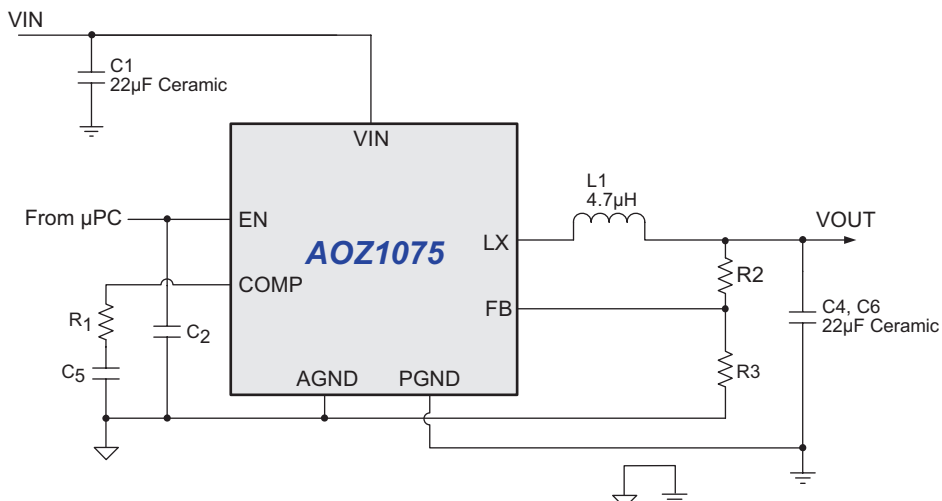
Figure 1. 3.3V/1.2A Buck Regulator
