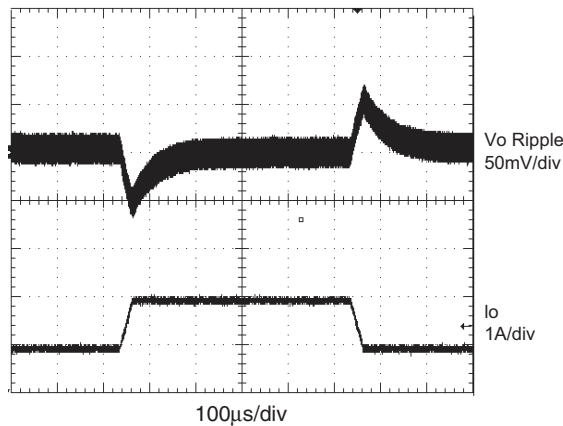
10% to 100% Load Transient
