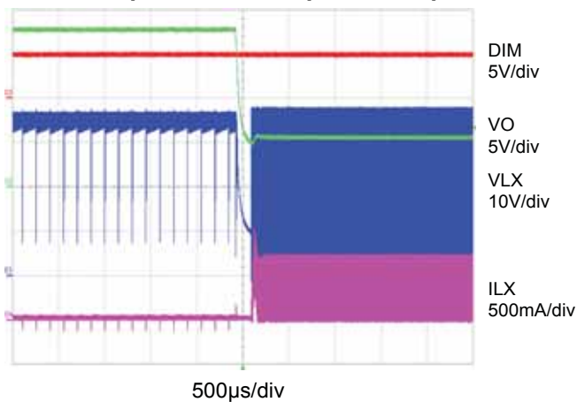
LED Open to Normal (36V/3 LED)
