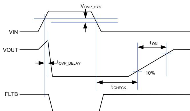
Figure 3. Over-voltage Protection (-01)
