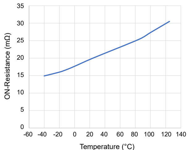
Figure 16. ON-resistance vs. Temperature
