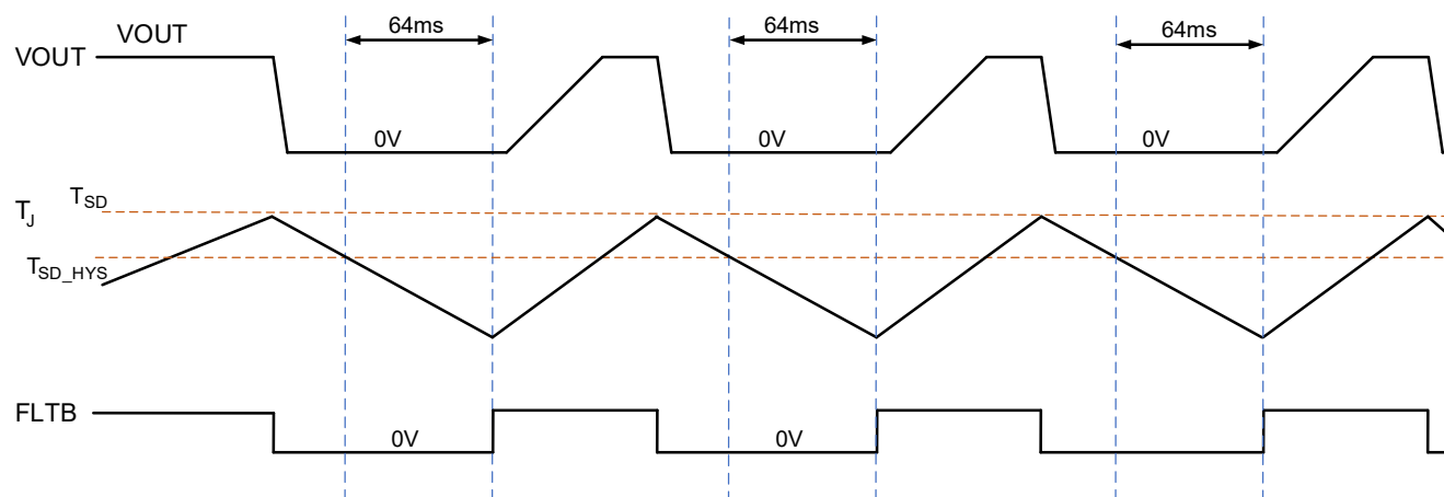
Figure 11. Thermal Shutdown (-01)
