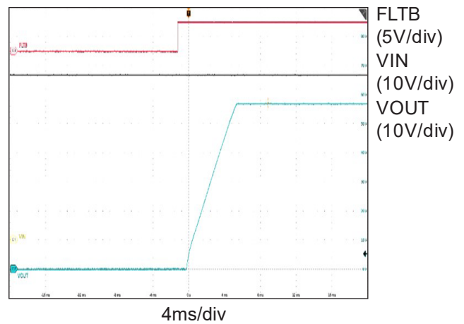
Over-voltage Protection ( R_{OVP} = 300k )
