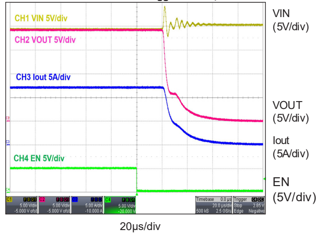
Shut Down (VIN = 20V, Load = 12A Pure Resistive Load, CSS = 5.6nF)
