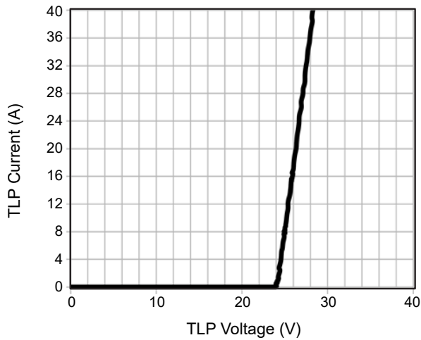
Figure 10. Positive Curve IEC61000-4-5 Surge 8/20µs
