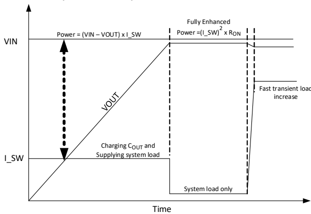
Figure 15. Soft-Start Power Dissipation
