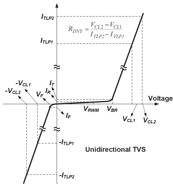
Figure 3. TVS Voltage vs. Current
