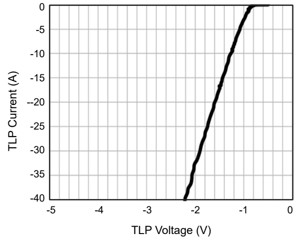
Figure 11. Negative Curve IEC61000-4-5 Surge 8/20µs
