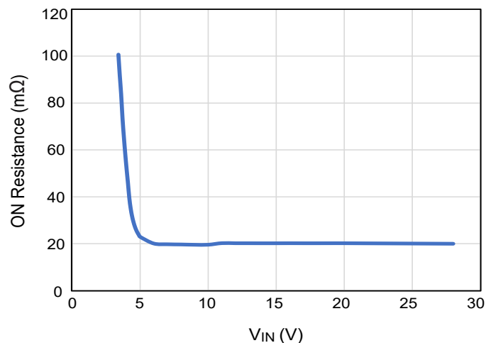
On Resistance vs. V_{IN}
