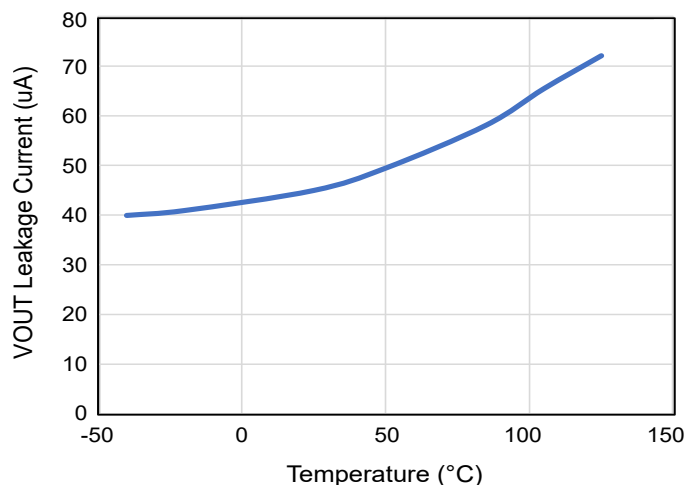
V_{OUT} Leakage Current vs. Temperature
