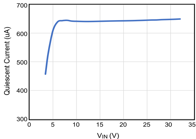
Quiescent Current vs. V_{IN}
