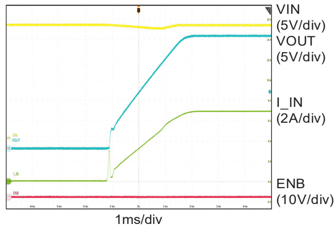
Soft Start Ramp ( V_{IN}=28\text{V} , 4\text{ohm CR load} )
