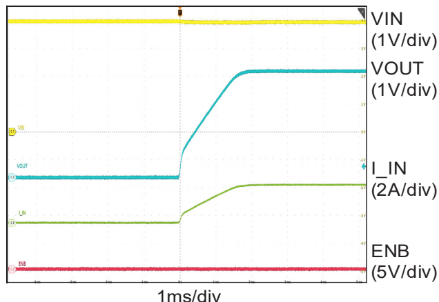
Soft Start Ramp ( V_{IN}=4\text{V} , 1.5\text{ohm load} )
