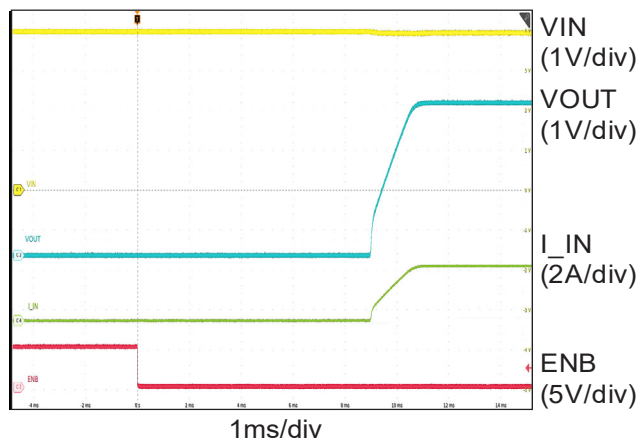
Soft Start Delay Time ( V_{IN}=4\text{V} , 1.5\text{ohm load} )
