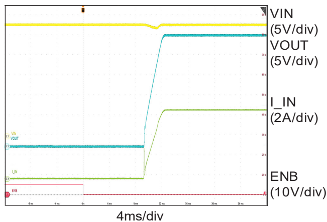
Soft Start Delay Time ( V_{IN}=28\text{V} , 4\text{ohm CR load} )
