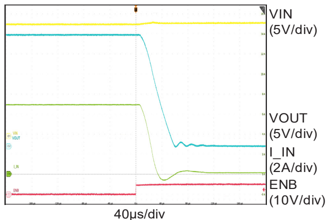
Shut Down ( V_{IN}=28\text{V} , 4\text{ohm CR load} )
