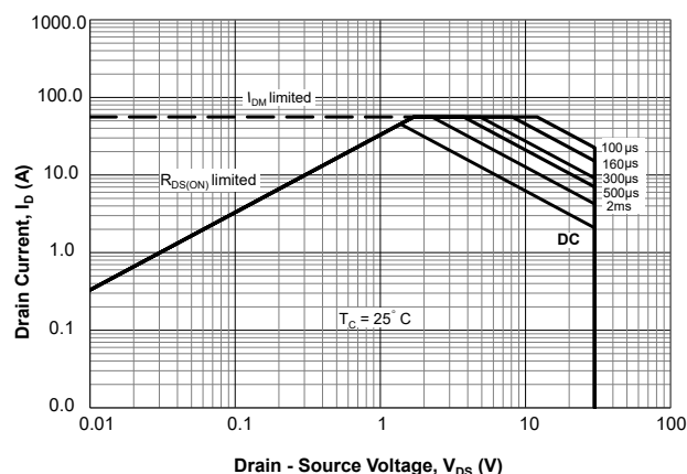
Figure 4. Safe Operating Area (SOA) Curves for Power Switch
