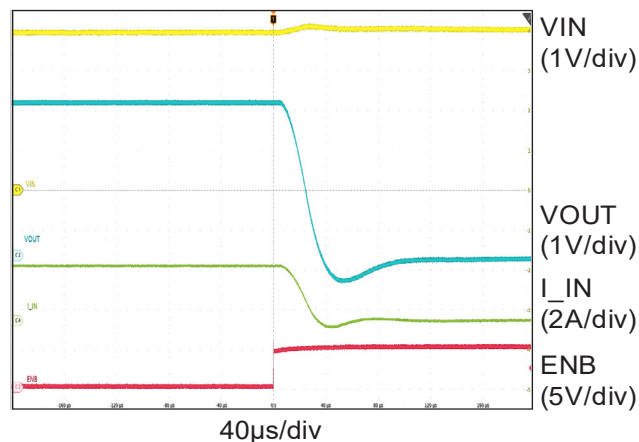
Shut Down ( V_{IN}=4\text{V} , 1.5\text{ohm load} )
