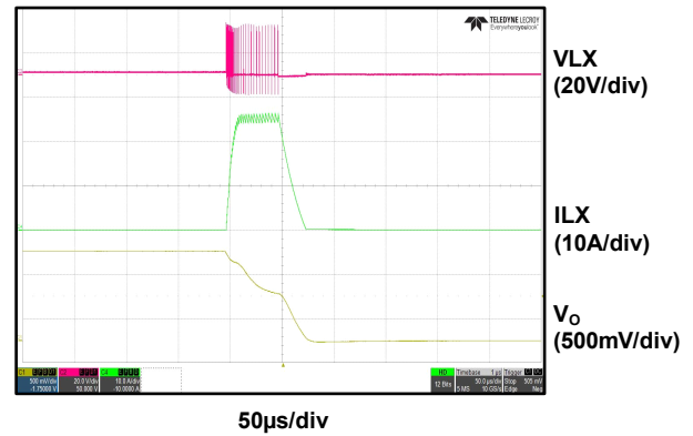
Short Circuit Protection (20kΩ ROCS)
