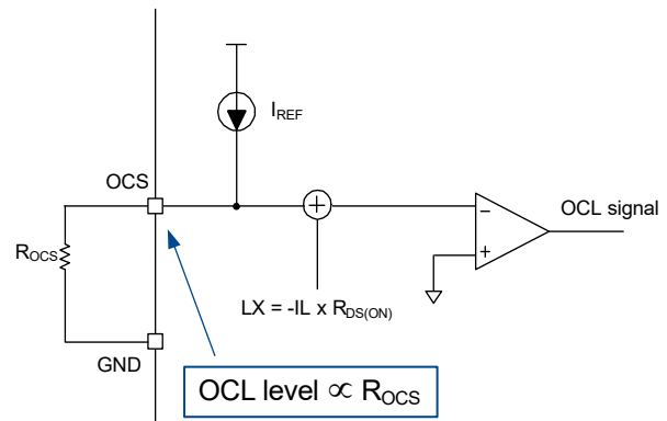
Figure 4. Illustration of Current Limit Setting
