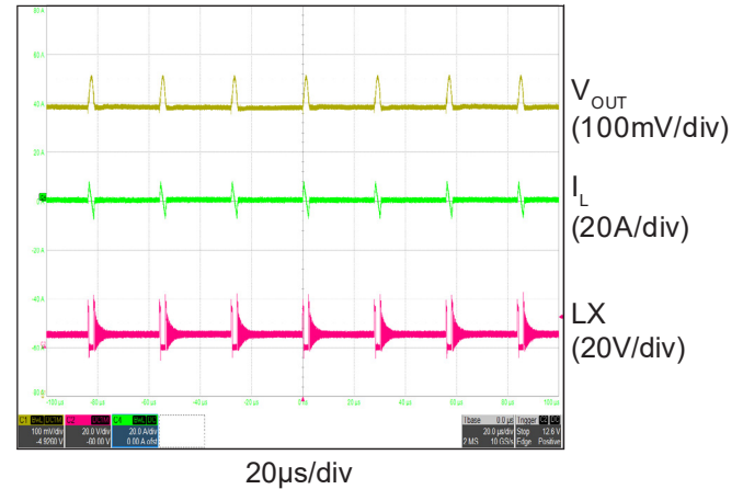
Ultrasonic Mode ( V_{IN} = 9\text{V} , I_{OUT} = 0\text{A} )
