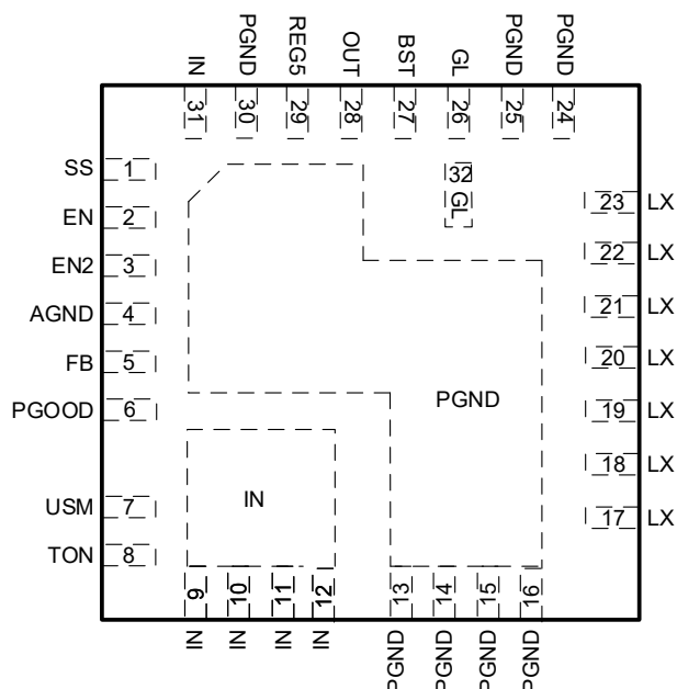
AOZ2297QI-05 31-Pin 4mm x 4mm QFN
