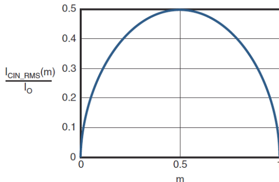
Figure 9. I_{CIN} vs. Voltage Conversion Ratio
