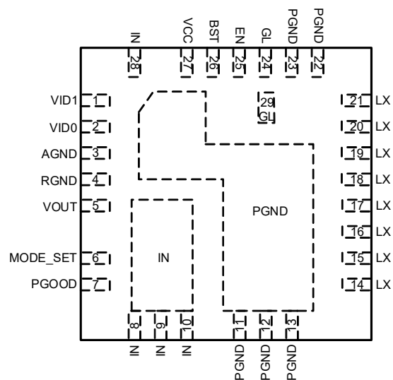
28-Pin 5mm x 5mm QFN (Top Transparent View)
