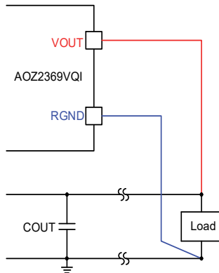
Figure 8. Decay Mode Illustration for Sleep Mode
