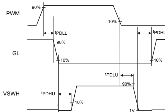
Figure 1. PWM Logic Input Timing Diagram
