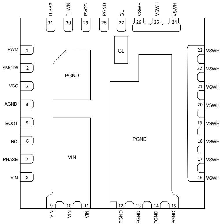
QFN5x5-31L (Top View)
