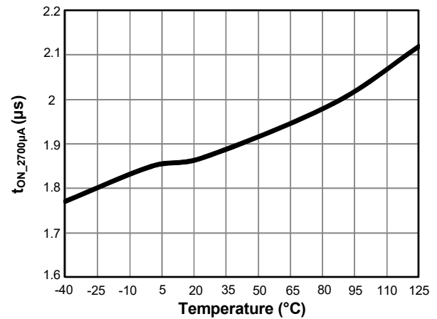
Figure 9. Time of TX signal (TXP to TXN)_2700μA vs. Temperature
