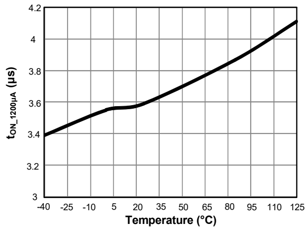
Figure 10. Time of TX signal (TXP to TXN)_1200μA vs. Temperature
