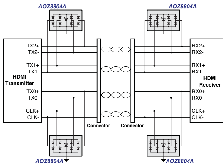
Figure 2. HDMI Ports
