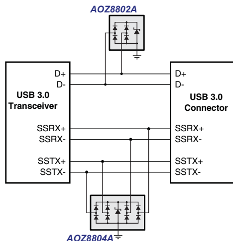
Figure 1. USB 3.0 Ports
