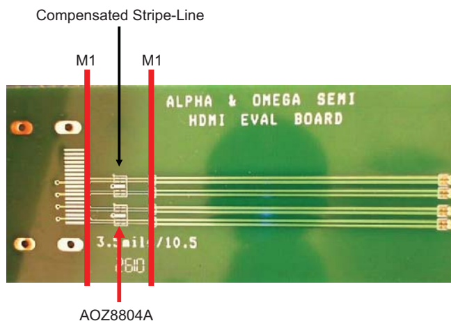
Figure 5. AOS HDMI Compensated Evaluation Board
