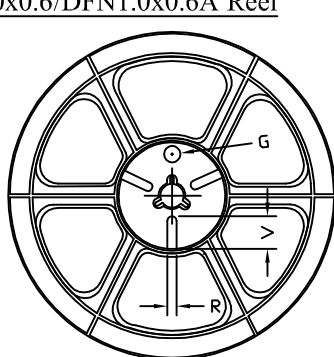
DFN1.0x0.6/DFN1.0x0.6A Reel
