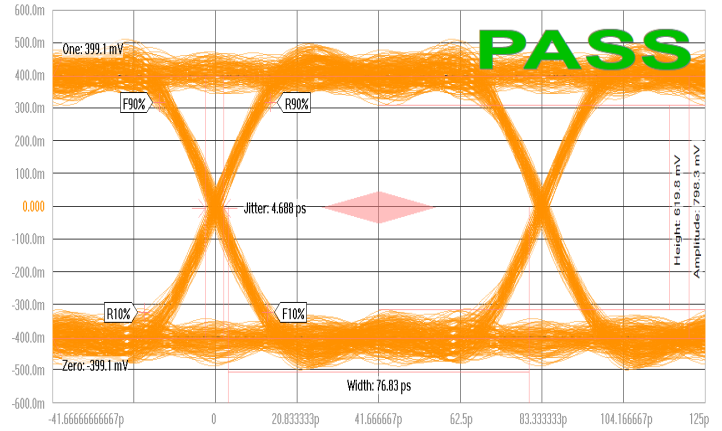
HDMI2.0 Eye Diagram (12 Gbps)
