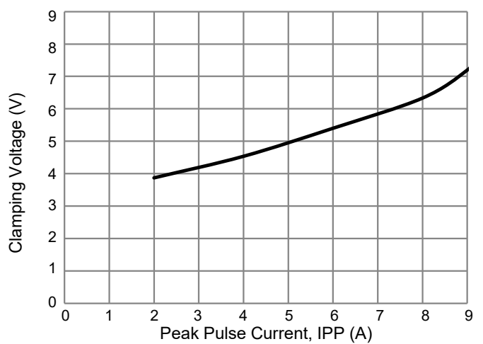
IEC61000-4-5 Surge 8/20μs (Any Pin to Pin)
