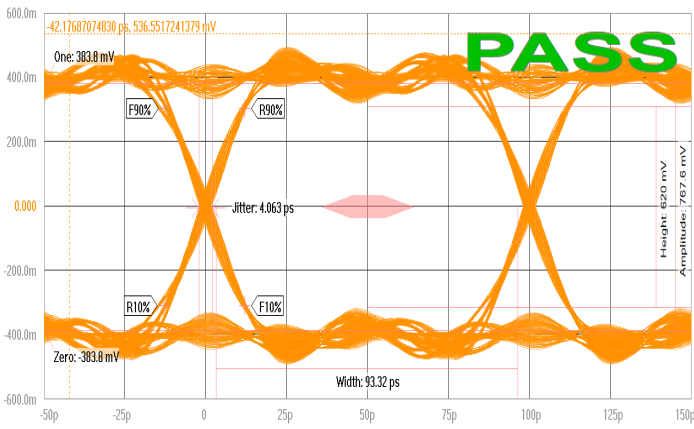
USB3.1 Gen2 Eye Diagram (10 Gbps)
