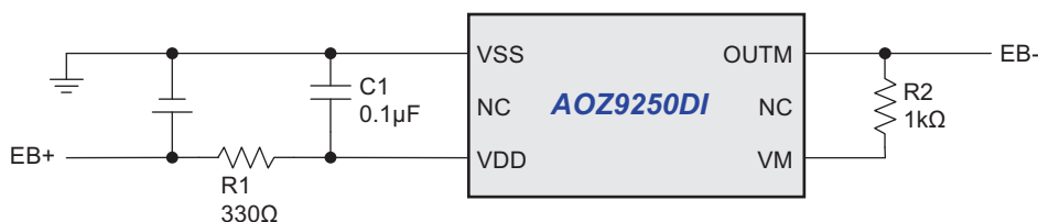
Figure 6. AOZ9250DI Applications Circuit
