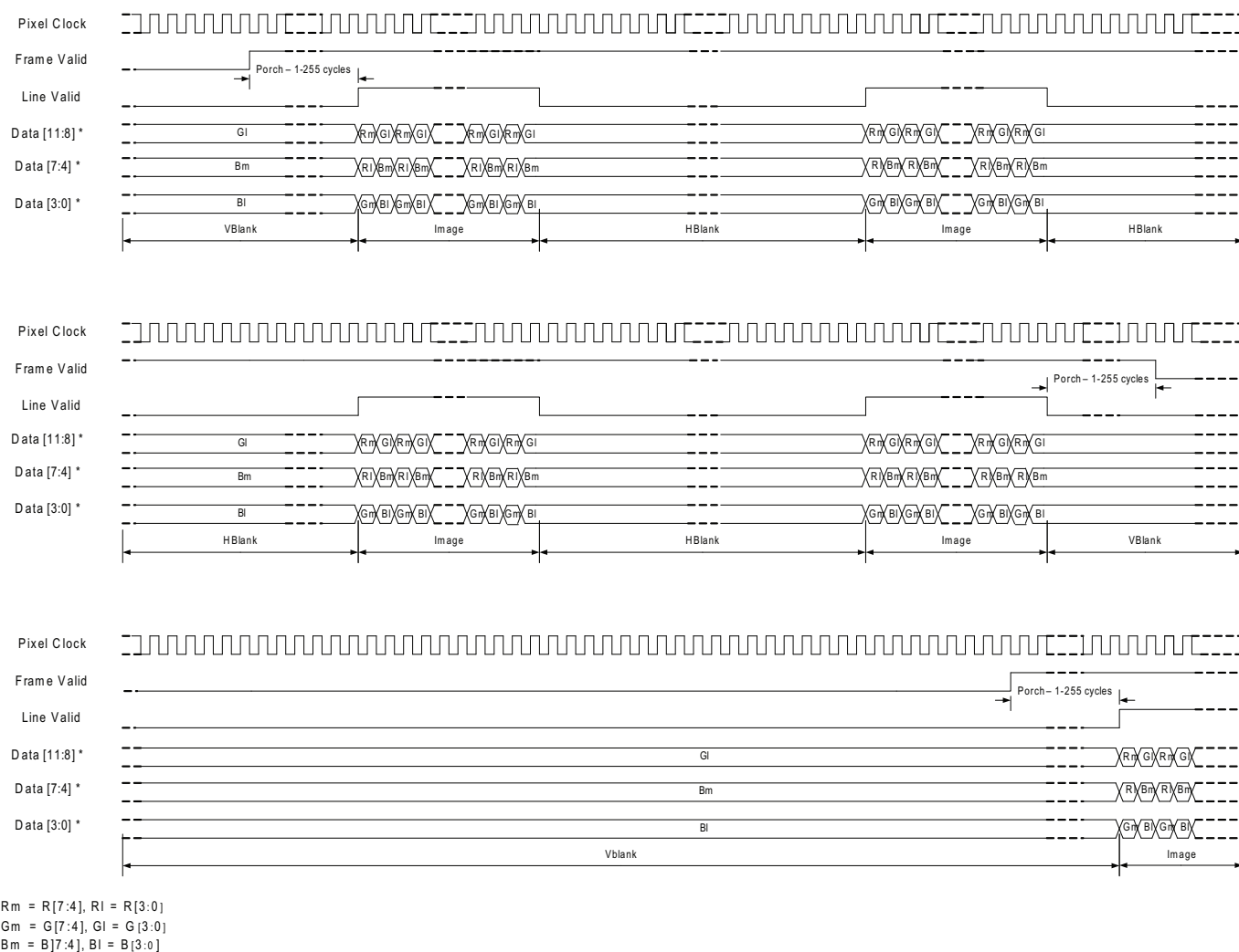
Figure 19: 12+12-bit RGB888 Output
