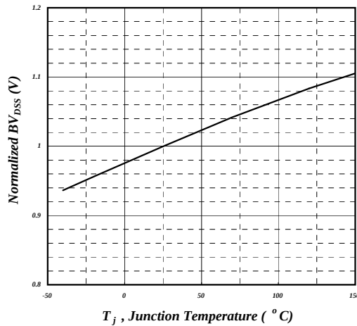
Fig 3. Breakdown Voltage vs. Junction Temperature
