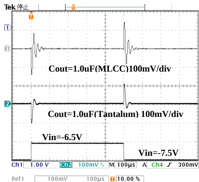
■Cin=1.0uF(Tantalum) Iout=100mA
