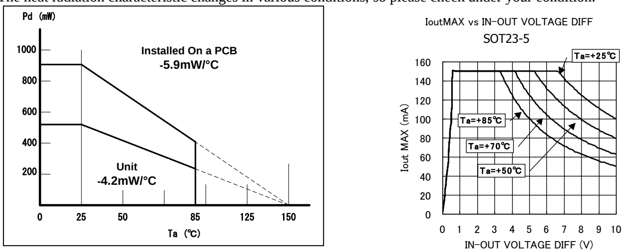
Figure 6. SOT23-5
