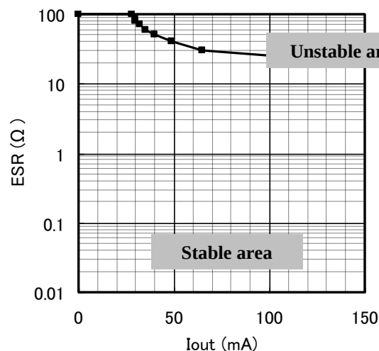
Figure 2. Stability area graph Condition: V_{in}=V_{out}(typ)-1.5V C_{in}=0.1\mu F , C_{out}=1.0\mu F (MLCC)
