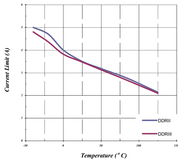
Source Current Limit vs Temperature
