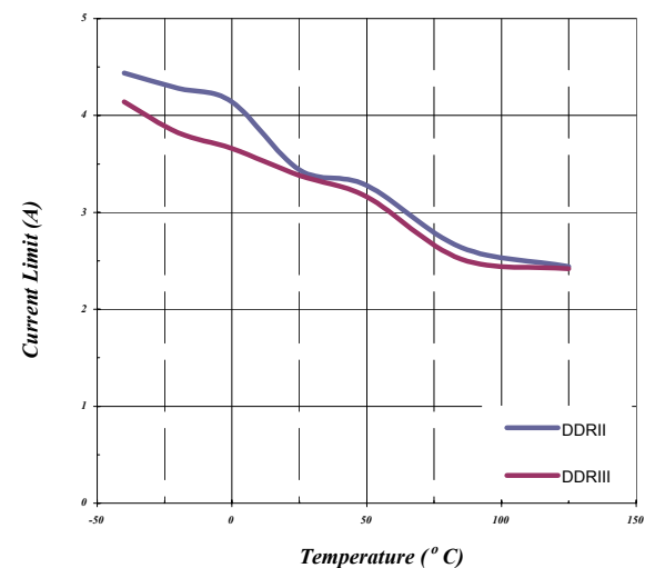
Sink Current Limit vs Temperature
