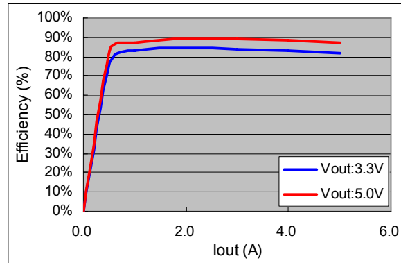
Efficiency (Vin = +12V)
