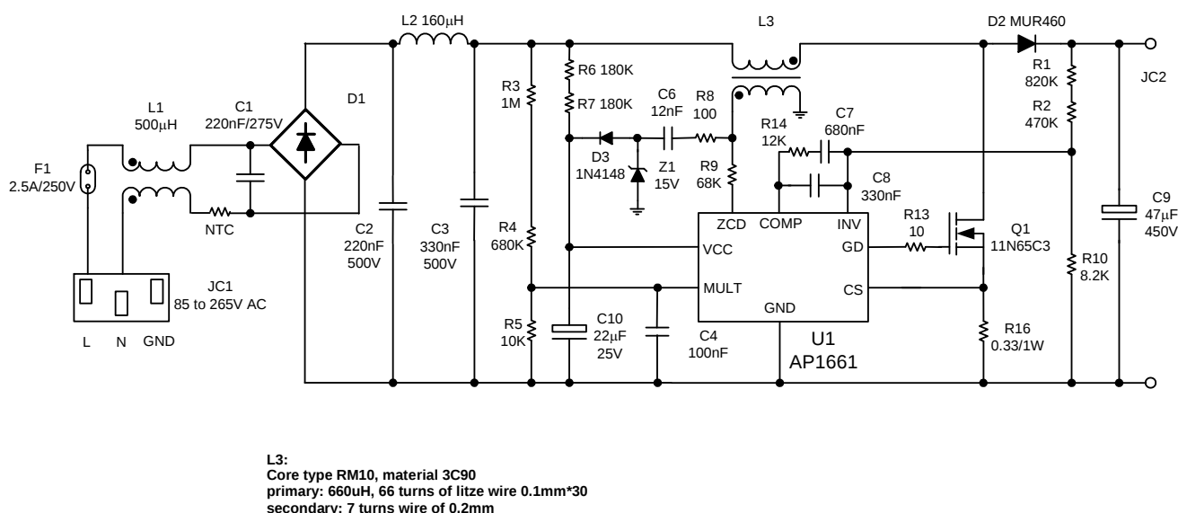
Figure 12. 85 to 265V Wide Range Input 90W PFC Demo Board Electrical Schematic Circuit
