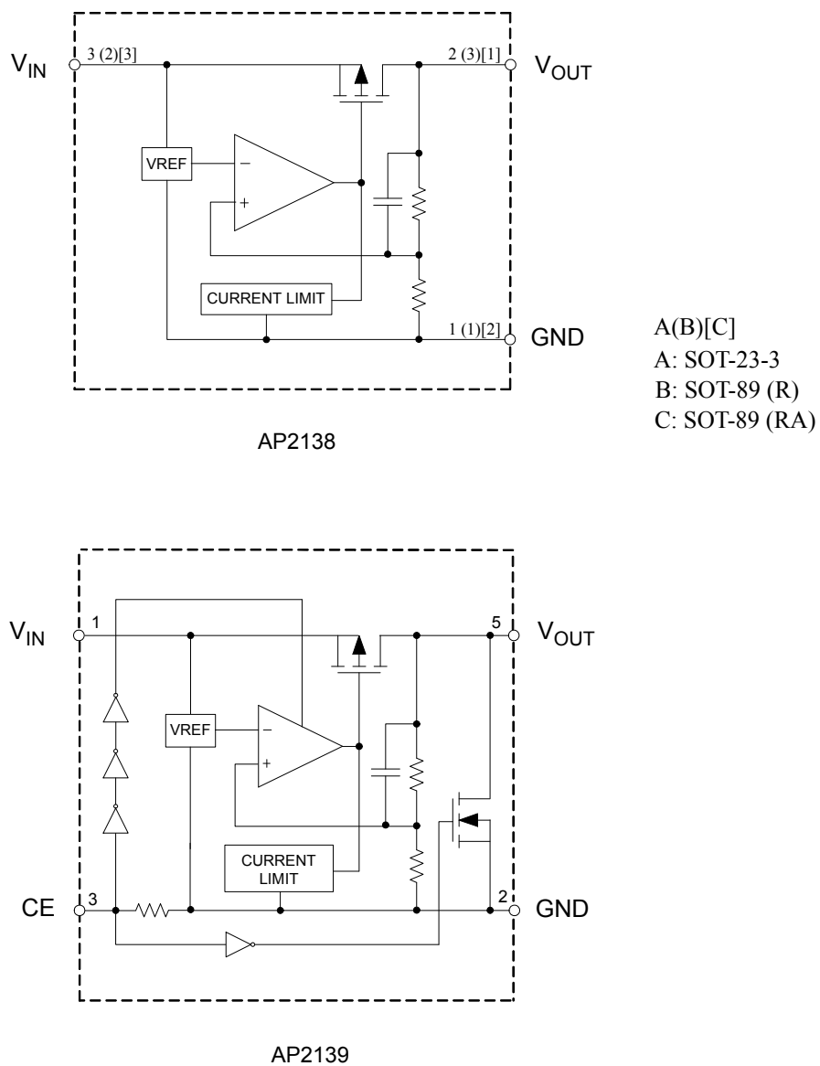
Figure 3. Functional Block Diagram of AP2138/2139
