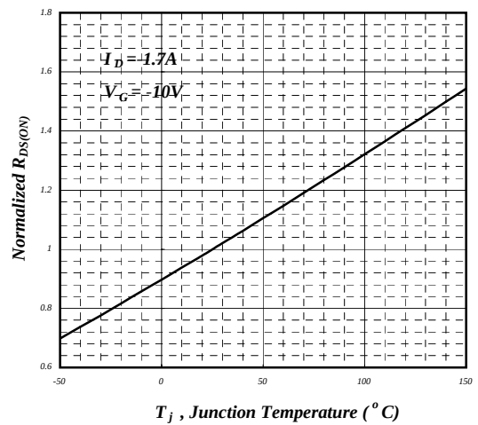
Fig 4. Normalized On-Resistance
