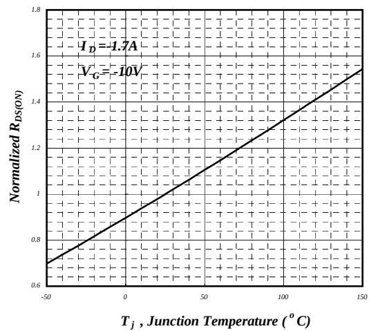
Fig 4. Normalized On-Resistance
