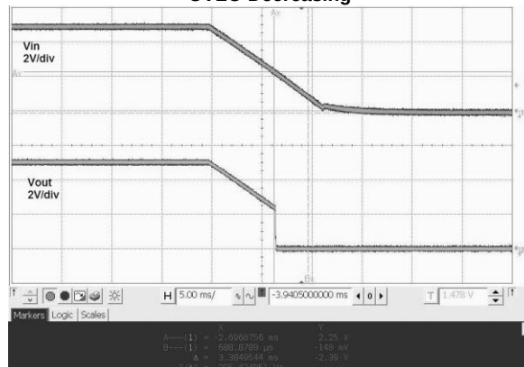
UVLO Decreasing
