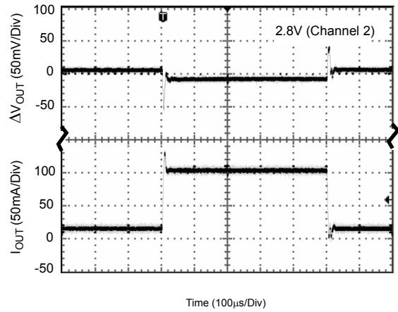
Figure 39. Load Transient
