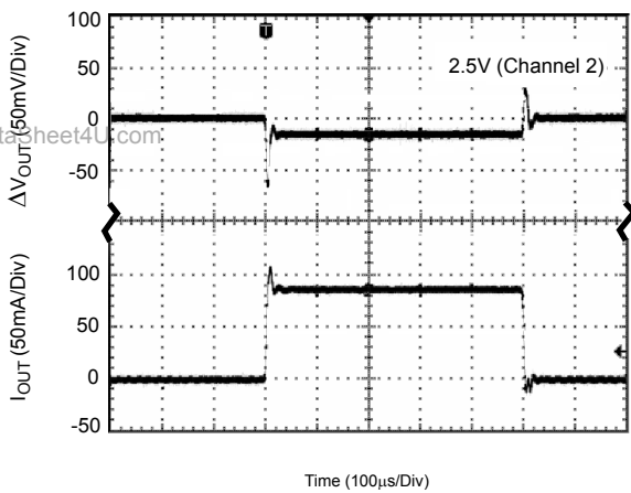
Figure 38. Load Transient
