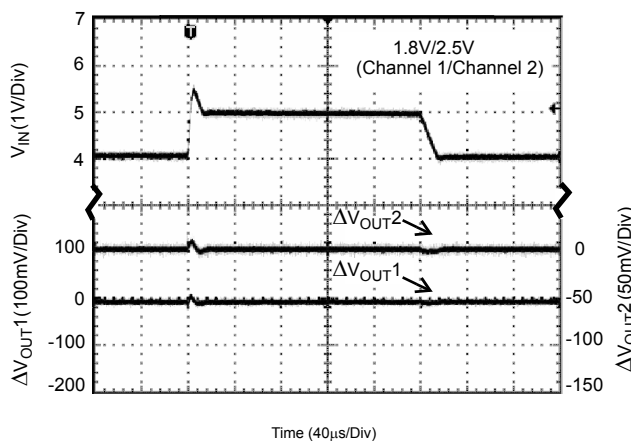
Figure 36. Line Transient
