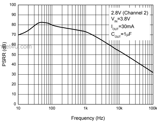
Figure 54. PSRR vs. Frequency
