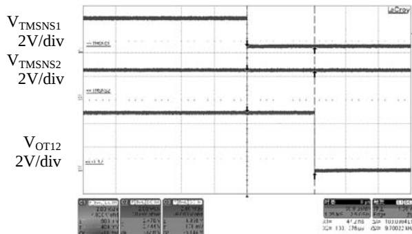
Figure 14. Deglitch Time to OT Low ( V_{SEL}=GND ) (Conditions: V_{CC}=5V , V_{TMSNS1}=0.5V to 3V , V_{TMSNS2}=2.5V , V_{TRIG}=1V )
