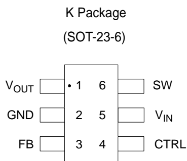
Figure 2. Pin Configuration of AP3019 (Top View)
