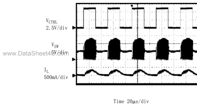
Figure 21. High Frequency (25kHz) Dimming Waveform
