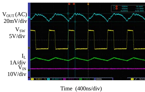
Figure 10. Output Ripple ( I_{OUT}=1.5\text{A} )
