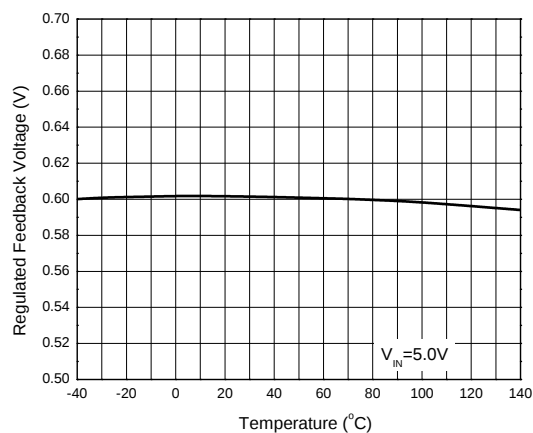
Regulated Feedback Voltage vs. Temperature
