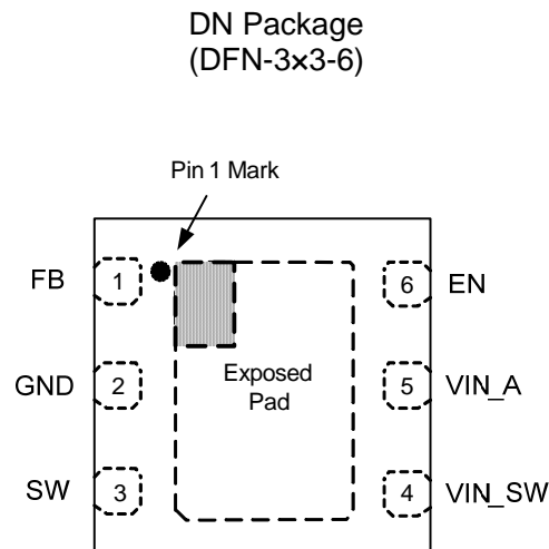
Figure 2. Pin Configuration of AP3432 (Top View)
