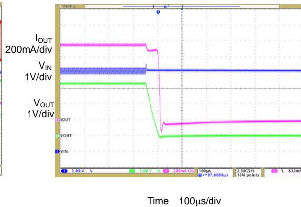
Figure 27. OTP Function
