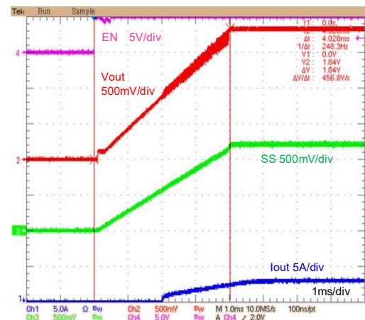
Figure 13. Soft Start
