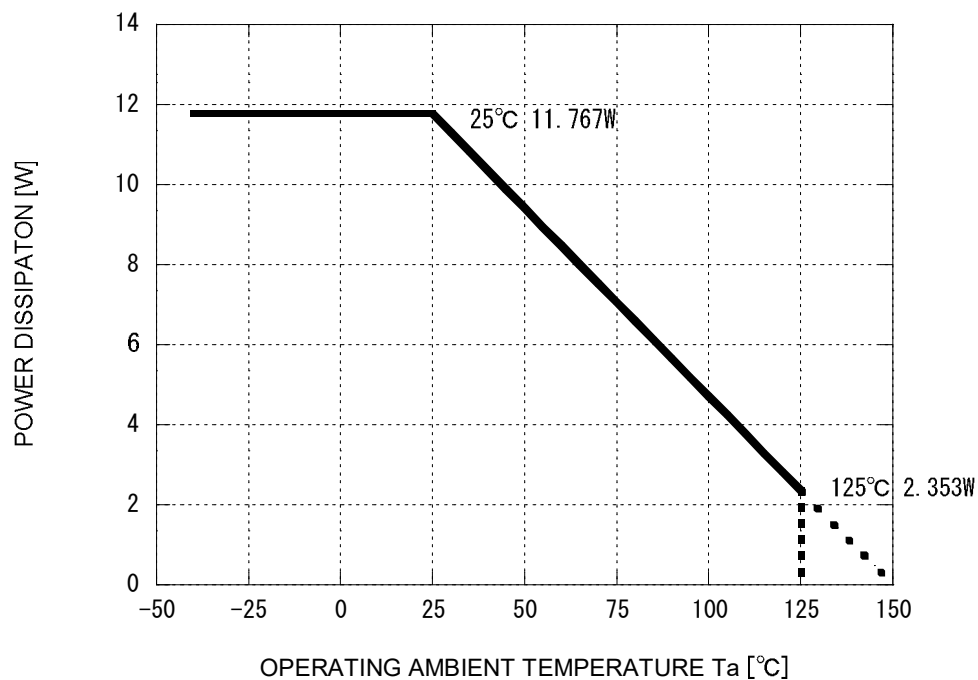
Figure 4. Power Dissipation
