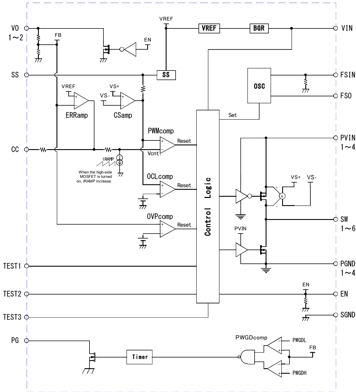
Figure 2. Block Diagram
