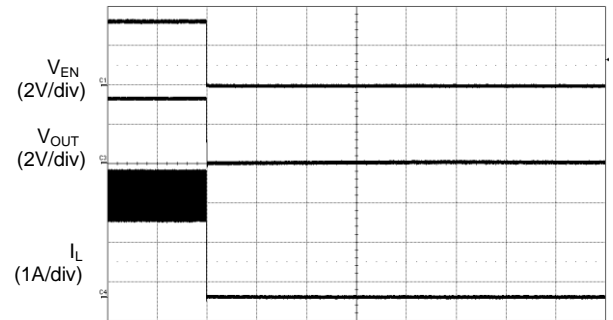
Power Off from EN ( I_{OUT} = 2.5A )
