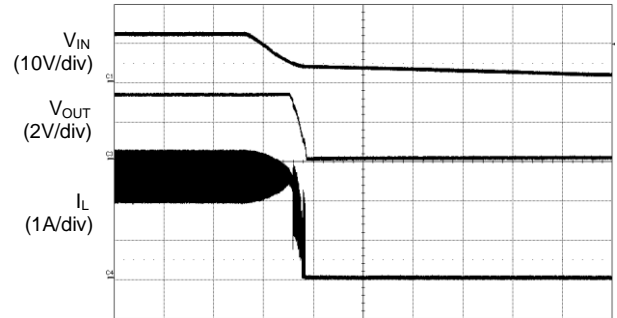
Power Off from VIN ( I_{OUT} = 2.5A )
