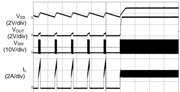
Short Circuit Protection Recovery ( I_{OUT} = 2.5A )
