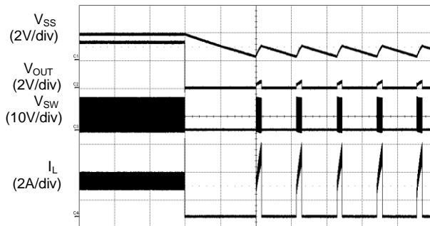
Short Circuit Protection ( I_{OUT} = 2.5A )
