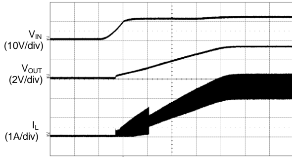
Power On from VIN ( I_{OUT} = 2.5A )
