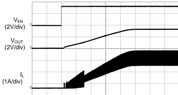
Power On from EN ( I_{OUT} = 2.5A )
