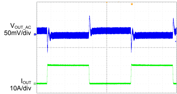
Time 400µs/div
