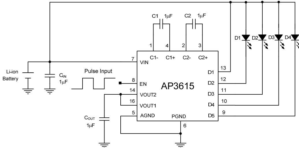
4 WLEDs
