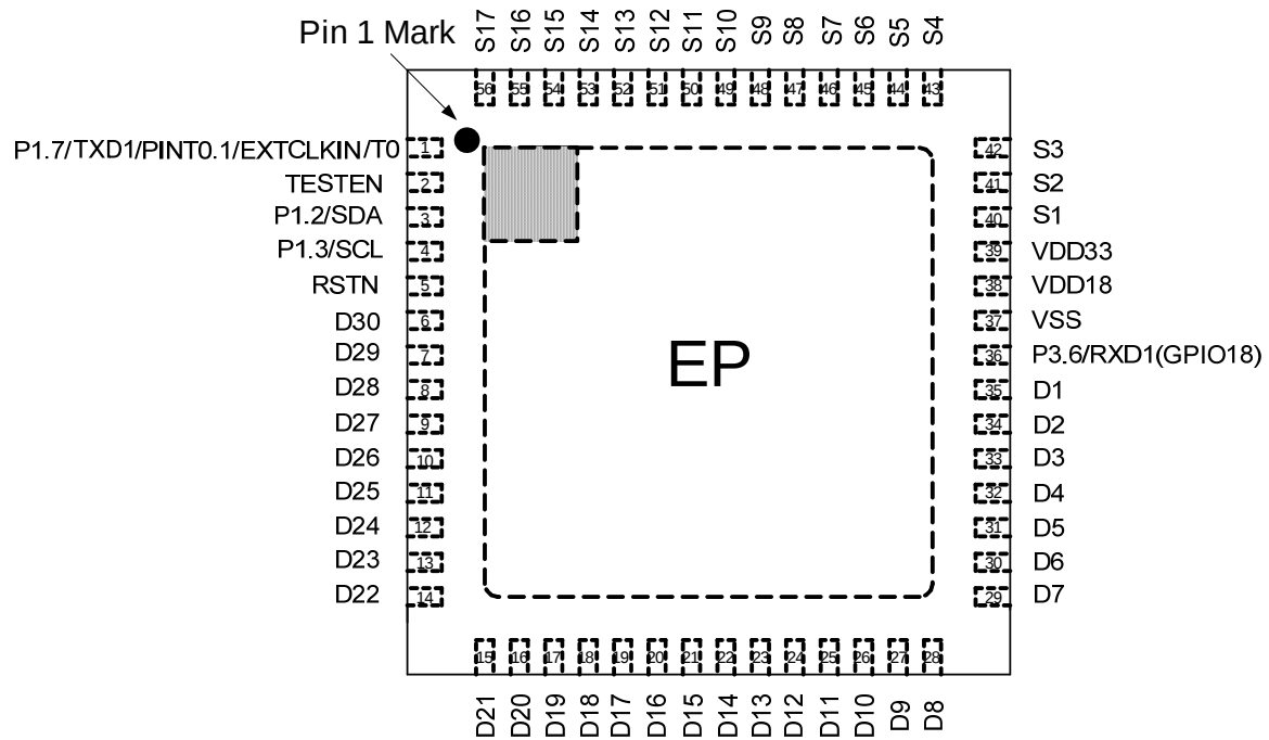
Figure 2. Pin Configuration of AP3890 (Top View)
