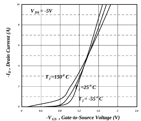
Fig 12. Transfer Characteristics
