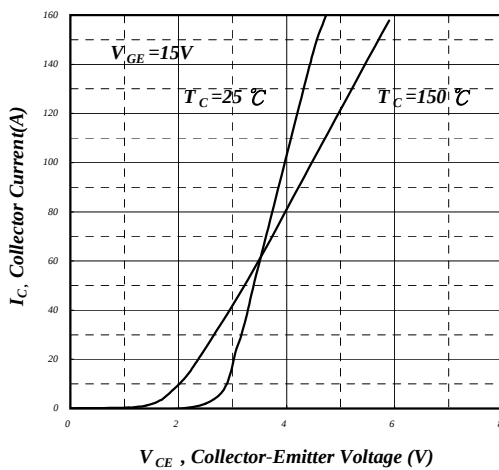
Fig 3. Typical Saturation Voltage Characteristics
