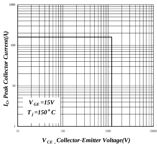
Fig 7. Revers Bias SOA
