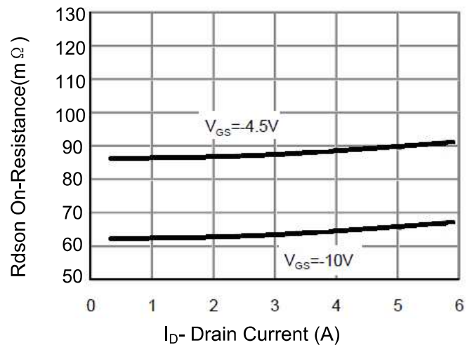
Figure 4 Drain-Source On-Resistance
