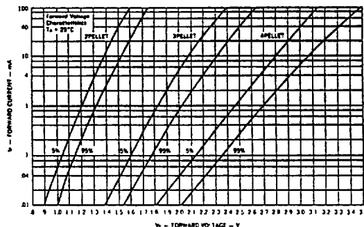
Figure 1 FORWARD VOLTAGE vs CURRENT
