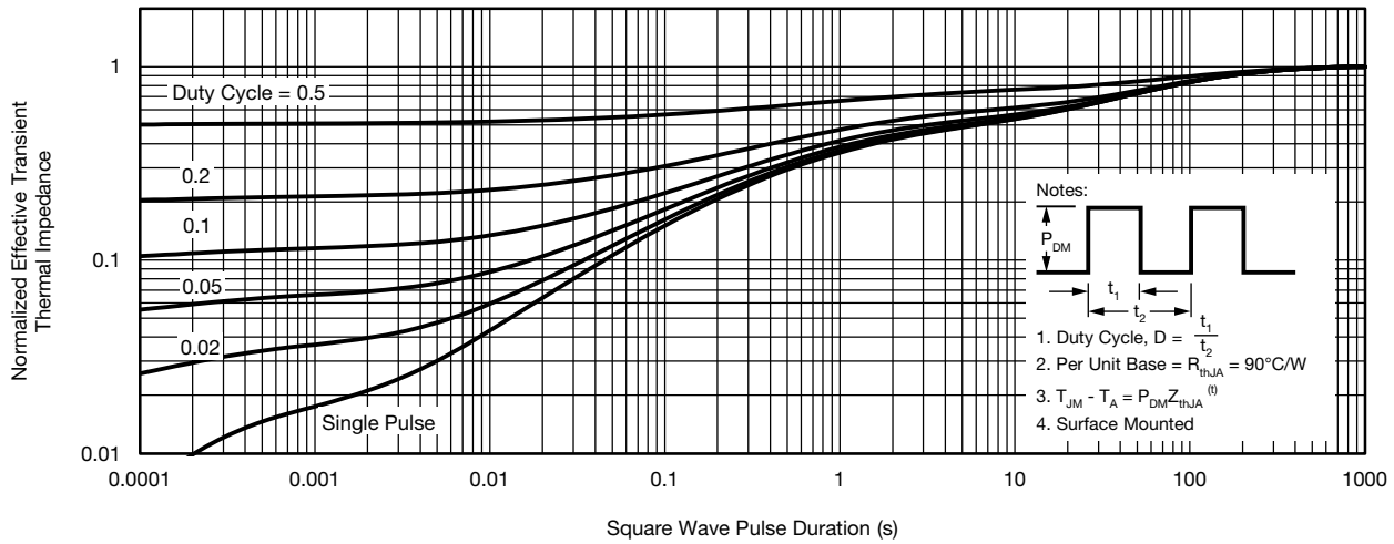
Normalized Thermal Transient Impedance, Junction-to-Ambien
