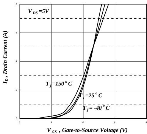
Fig 11. Transfer Characteristics
