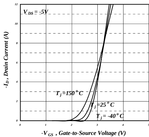
Fig 11. Transfer Characteristics
