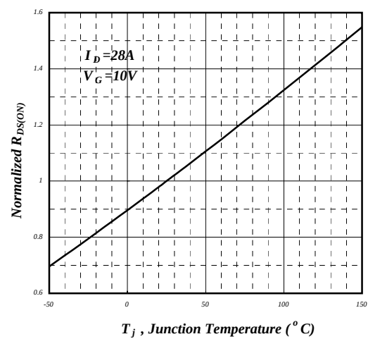
Fig 4. Normalized On-Resistance
