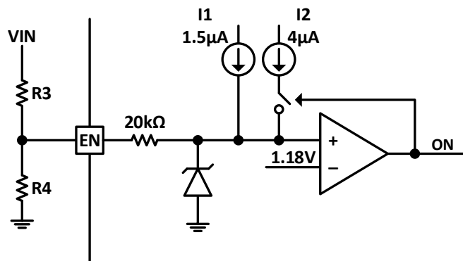
Figure 25. Adjusting UVLO
