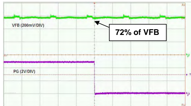
Time- 1µs/div Powergood Falling Threshold
