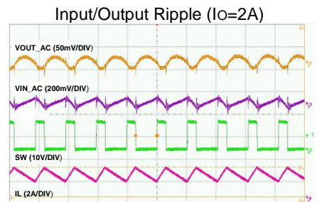
Time-2μs/div
