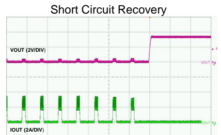
Time-5ms/div
