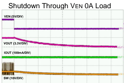
Time-500ms/div
