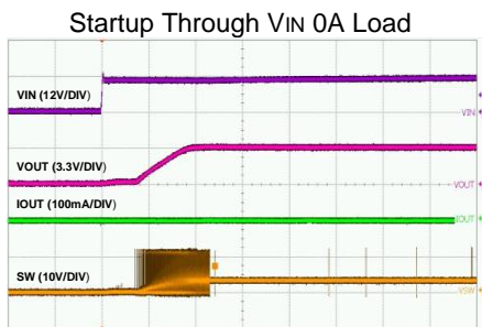
Time-500μs/div
