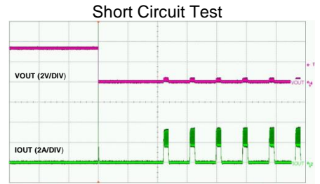
Time-5ms/div
