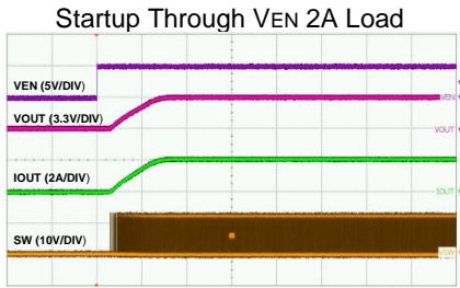
Time-500μs/div
