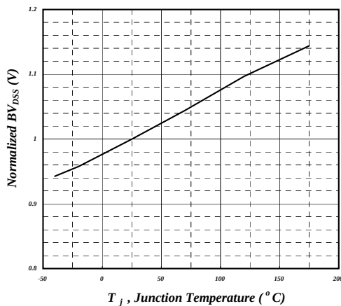
Fig 3. Normalized BV_{DSS} v.s. Junction Temperature
